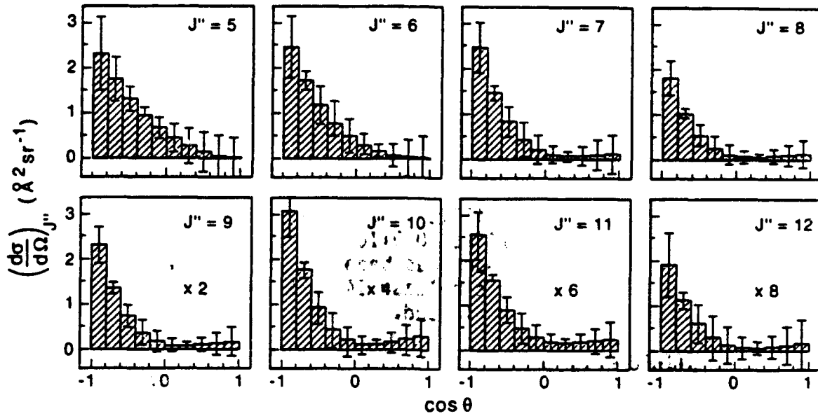
Fig. 12. Absolute differential cross sections (in Å 2 /steradian) for scattering of thermal HCl into a final J'' level. Note the strong propensity for cos(θ) = -1, i.e. predominantly forward scattering of the Cl atoms in the center-of-mass frame
